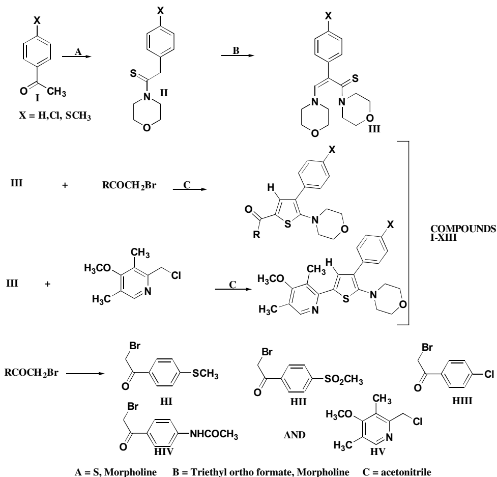
Scheme 1. Synthesis of trisubstituted thiophenes. The adduct III was reacted with various haloketones of the formula (HI–HIV) and 2-chloromethyl-3,5-dimethyl-4-methoxy-pyridine (HV) to yield the desired products of the formula (I–XIII).
