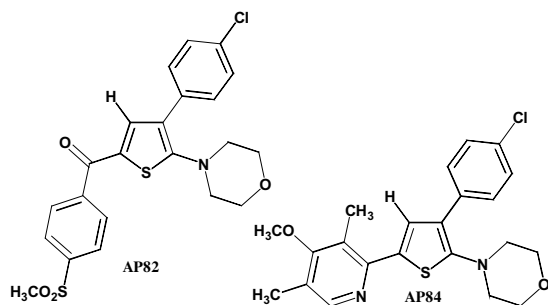
Figure 1. Trisubstituted thiophene AP82 and AP84 designed and synthesized as anti-inflammatory agents. AP82 had an aroyl substitution at the fifth position of the thiophene and AP84 had a pyridyl substitution at the fifth position.
